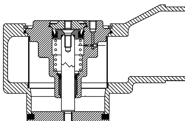
Section View of Assembly
