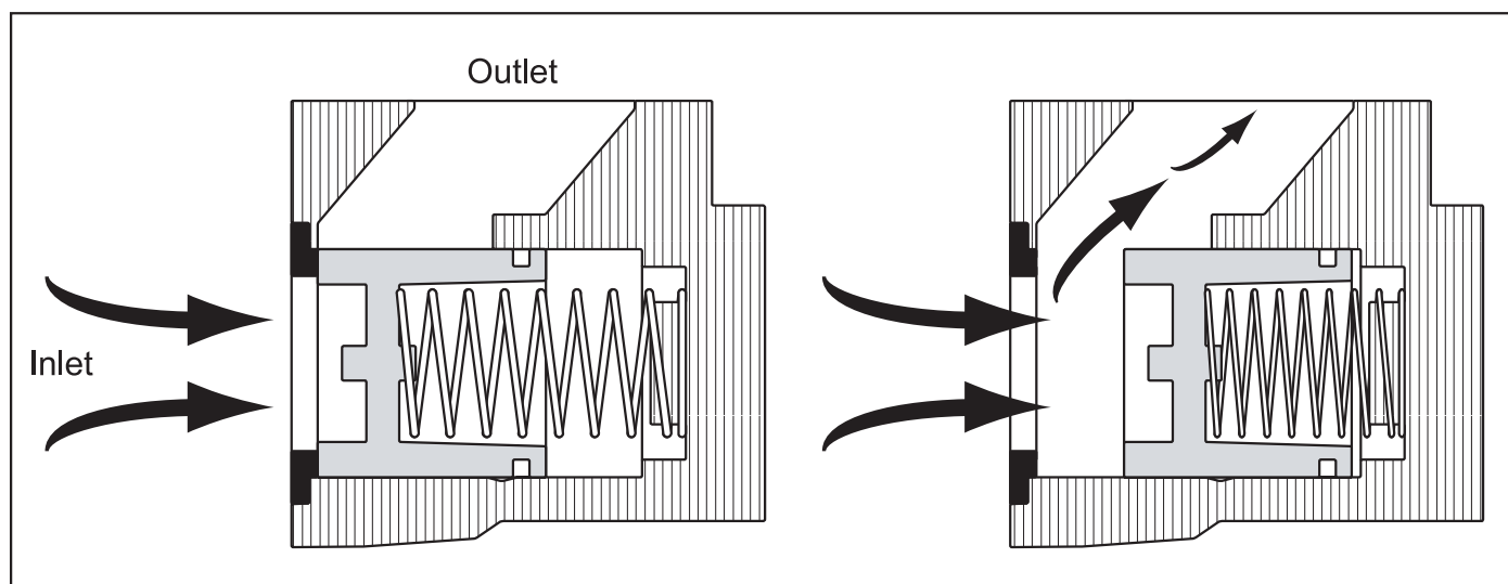
K-7 Valve Operation
